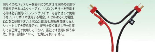
SGC-38 ¥460 バッテリー用 2 又直列 コネクタ 汎用 14AWG ▶ Two-pronged series connector for battery 14AWG (general purpose)
